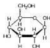
Figure 1 Glucose molecule
